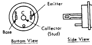
Flange Style Transistor - Type: 042, etc. Bottom View
