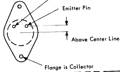
Flange Style Transistor - Type: 042, etc. Bottom View
