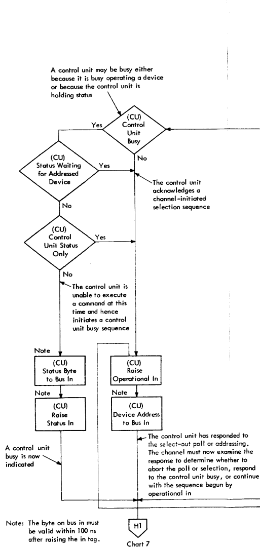
Control Unit Response to Select-Out -- Chart 6
