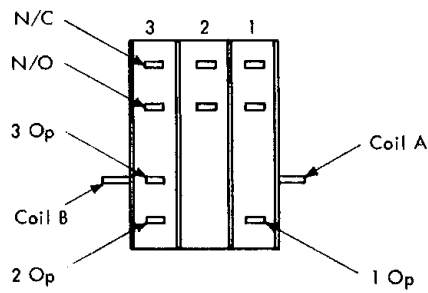
Relay (2 pole)
