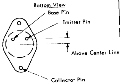
Flange Style Transistor - Type: 036, etc. Bottom View
